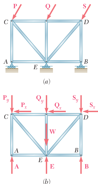
Fig. 4.6 Improper constraints.
