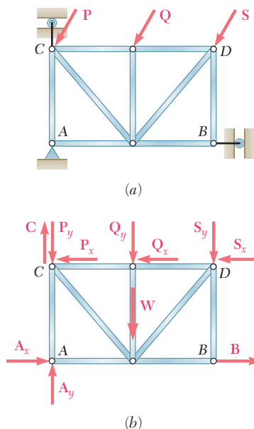
Fig. 4.7 Improper constraints.
