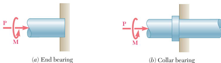
Fig. 8.11 Thrust bearings.
