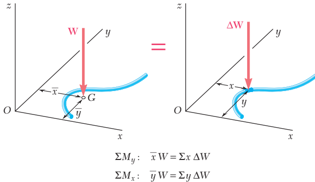
Fig. 5.2 Center of gravity of a wire.
